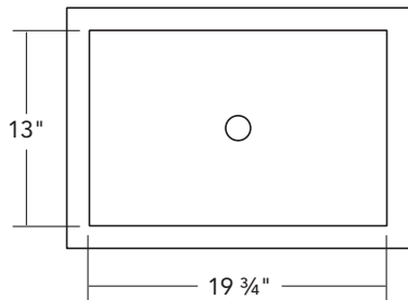
Basin inner dimensions
