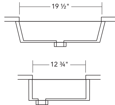
Sectional views
